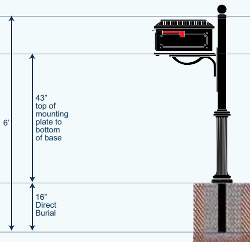
MODEL NUMBER FOR EXAMPLE SHOWN Wingate-FS-3SM-2-1017-1
