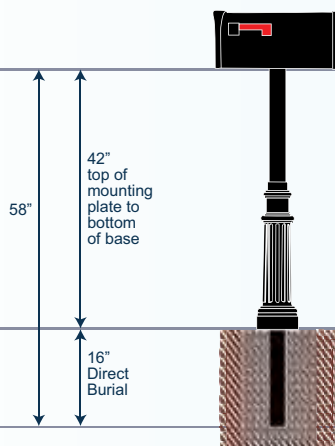
MODEL NUMBER FOR EXAMPLE SHOWN Bradford-TS-3SM-1008-5
