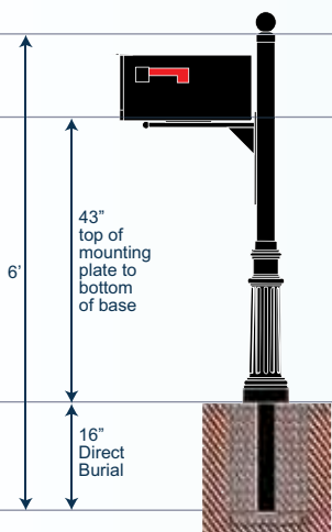
MODEL NUMBER FOR EXAMPLE SHOWN Ashley-FS-3SM-2-1018A-5
