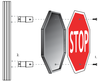
Back Plate, Sign Trim or Sign Frame mounting diagram (using TSB1 brackets)
