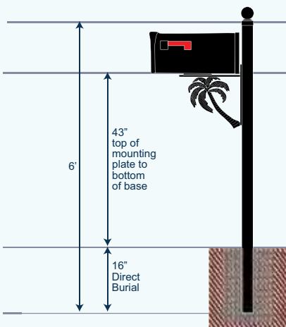
MODEL NUMBER FOR EXAMPLE SHOWN Palms-FS-3SM-2-1008
