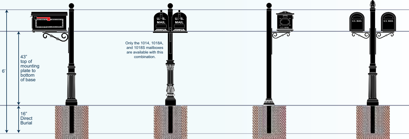
MODEL NUMBER FOR EXAMPLE SHOWN Bel-Aire-FS-3SM-2-1010-5
